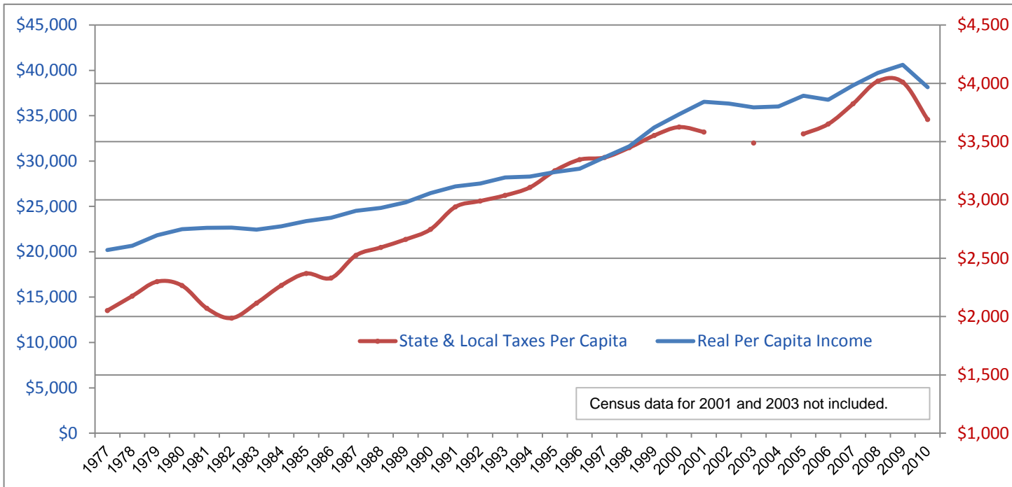
Chart 3. State and Local Taxes Per Capita Real Per Capita Income Washington Average 1976 - 2010
